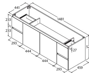
TOP VIEW: SHELF & DRAWER AREA (Dimensions may vary depending on basin position)
