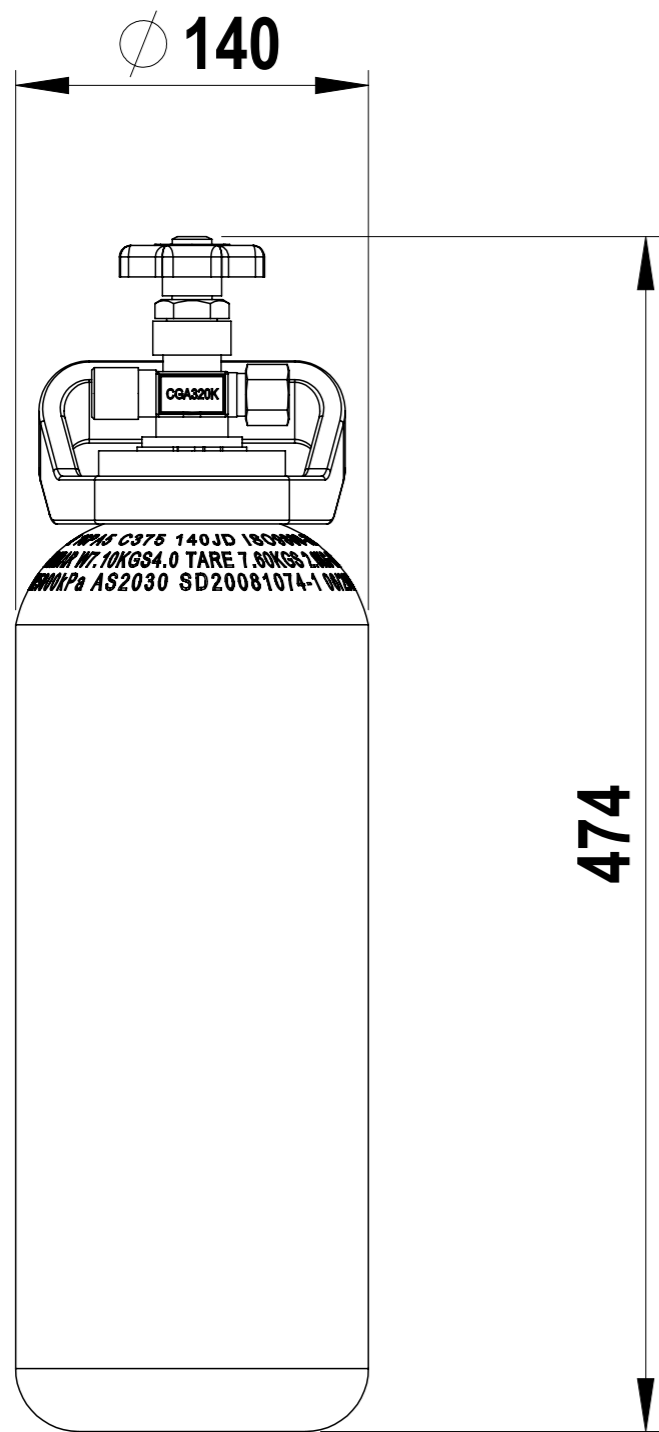
FRONT VIEW
