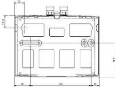
BACK VIEW SCALE 1:1.25
