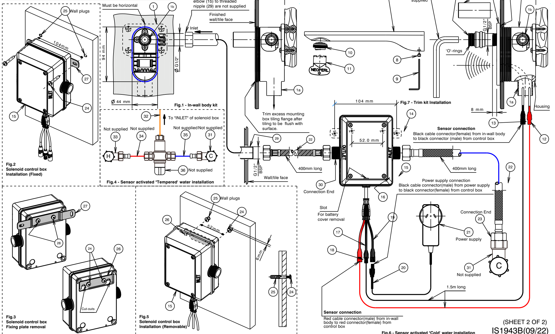
Fig.6 - Sensor activated "Cold" water installation
