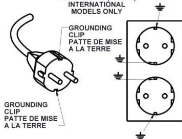
FIGURE C 230V NOMINAL / 50-60HZ 1-PHASE SHUKO CORD (TYPE F) INTERNATIONAL MODELS ONLY
