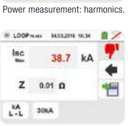
Advanced Loop: negative result of breaking capacity test.
