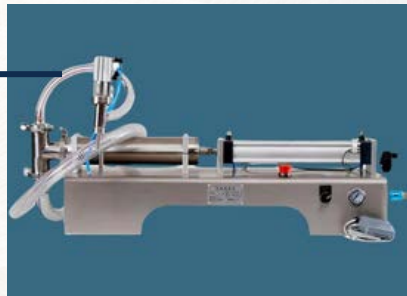
Horizontal Pneumatic Liquid Filling Machine (500-5000 ml)
