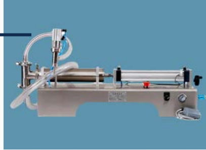
Horizontal Pneumatic Liquid Filling Machine (100-1000 ml)
