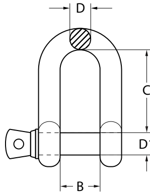
DEE SHACKLE
