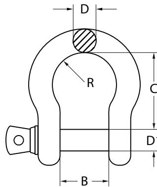
BOW SHACKLE
