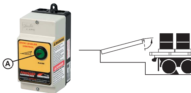
A—RAISE Button
