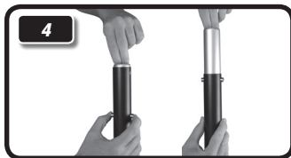
STEP 4 The built-in adapter fits both 1-1/2" or 1-3/8" internal diameter speaker sockets. Use the lower position for 1-1/2". For 1-3/8" sockets, depress push buttons and raise adapter until it locks in raised position.
