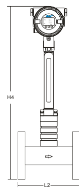
Flange Type
