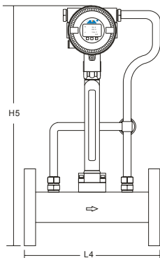
Flange Type with T/P Sensor
