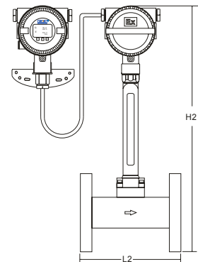
Remote Flange Type
