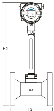
Reduced Bore Type
