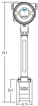
Wafer Type
