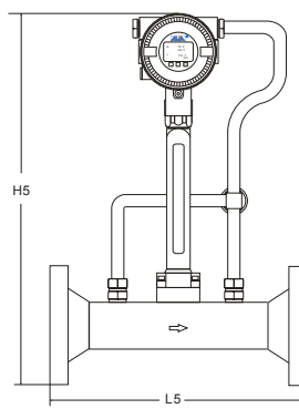
Reduced Bore Type
