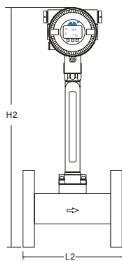
Flange Type
