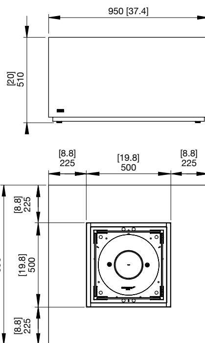
Line drawings show concrete models without a Fire Screen. Refer to the Fire Screen model specifications for dimensions.
