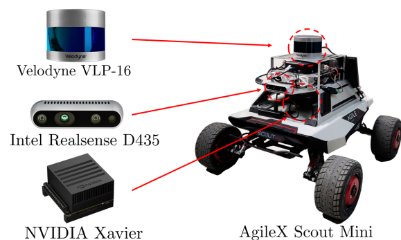
Figure 6. Mobile robotic platform equipped with 3D laser scanner, RGB camera and onboard computer.
