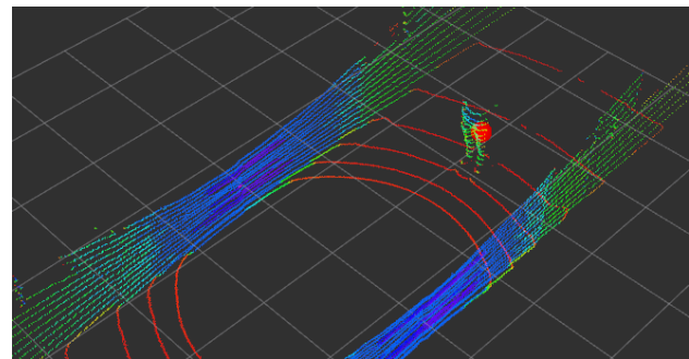
Figure 5. People positions in the LiDAR reference frame. The red marker represent the center of the three dimensional bounding box.
