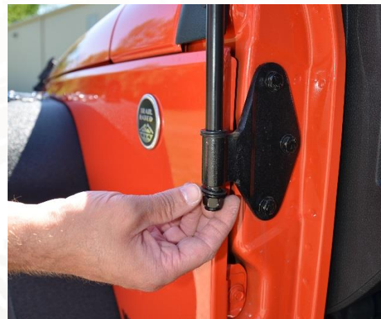
Figure 3: Install nylon washer, SS washer, then nyloc nut.
