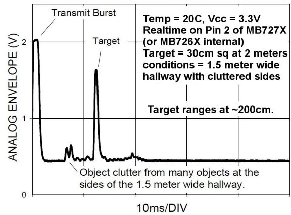
Analog Envelope Output (Clutter, 3.3V)
