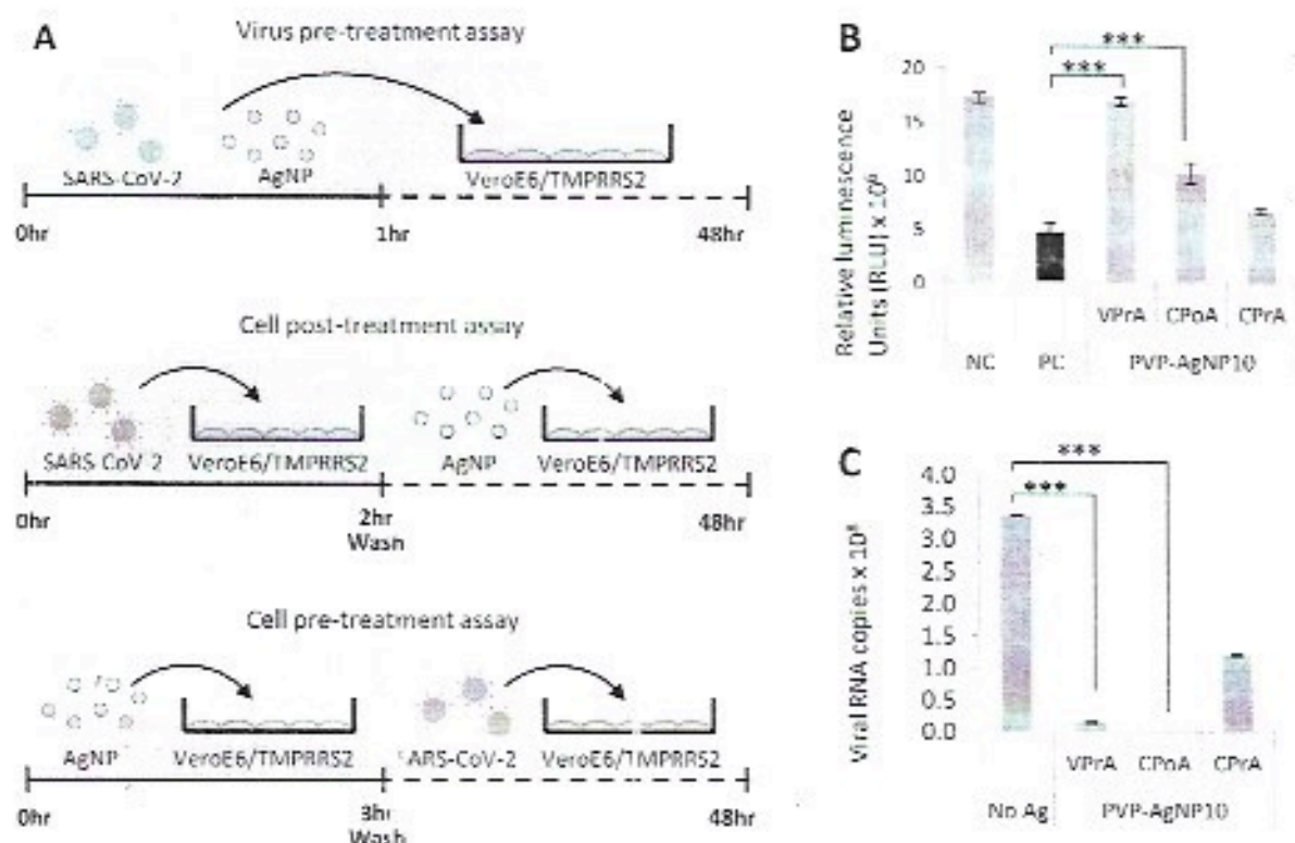
Fig. 3. Silver nanoparticles effectively inhibit extracellular SARS-CoV-2. 3A: Schematic representation of virus pre treatment assay (top panel), cell post-treatment assay (central panel) and cell pre-treatment assay (bottom panel). 3B: Performance of PVP coated 10 nm Silver nanoparticles in the three study designs with respect to rescue of cells from SARS-CoV-2 infection. Error bars obtained from triplicate testing. p value < 0.005 (***). 3C: Performance of PVP coated 10 nm Silver nanoparticles in the three study designs with respect to reduction of SARS-CoV-2 replication. Error bars obtained from triplicate testing. p value < 0.001 (***).
