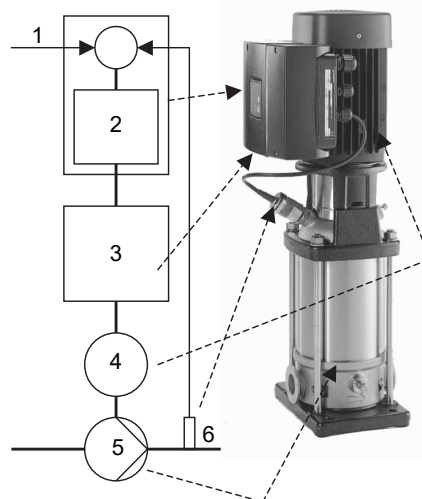
Components of a Grundfos E-pump
