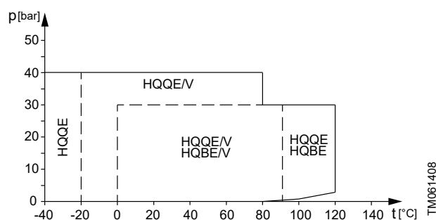
Operating range of standard shaft seals for CRE, CRIE, CRNE 1-155
