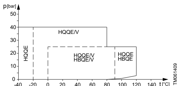
Operating range of standard shaft seals for CR, CRN 125-155
