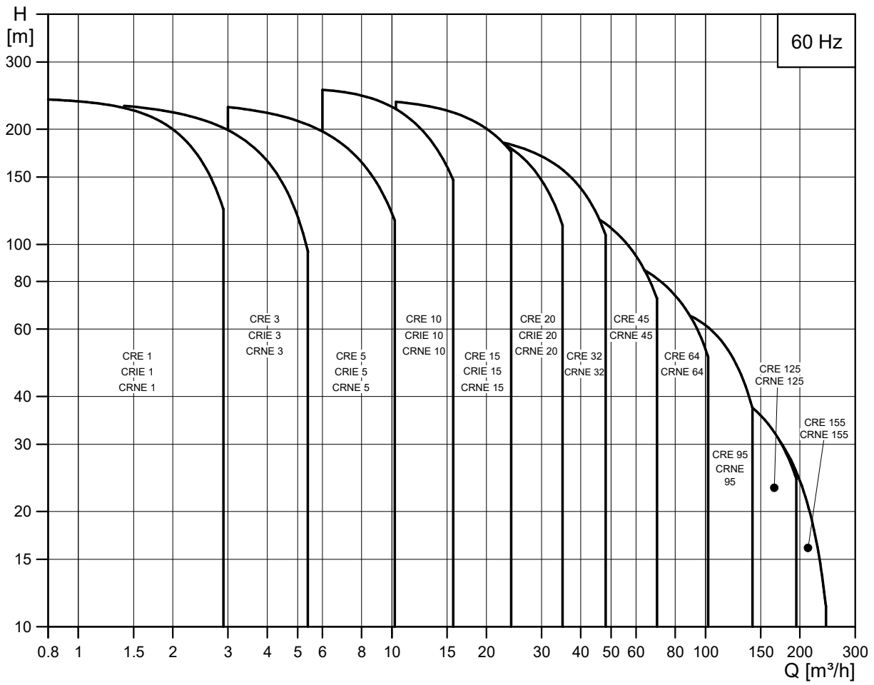
Performance range, CRE, CRIE and CRNE
