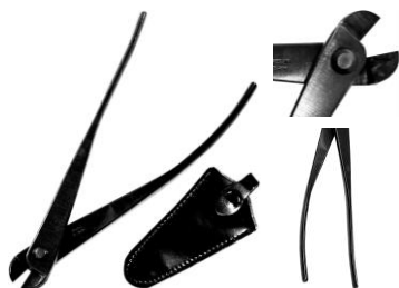
48045 GIKOH Bonsai Wire Cutter 205mm Overall Length (mm): 205 Blade Width (mm): 12 Weight (g): 100
