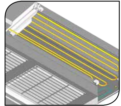
Piping foamed in place (all model 70 / 80)
