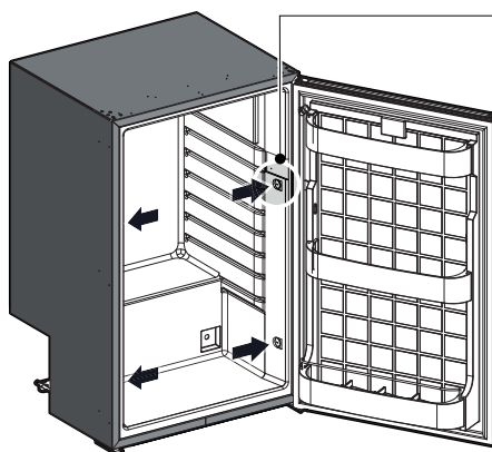
BOCCOLE INTERNE INTERNAL BUSHINGS
