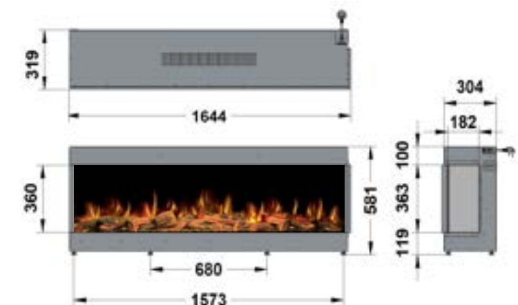
1650 - RIGHT CORNER
