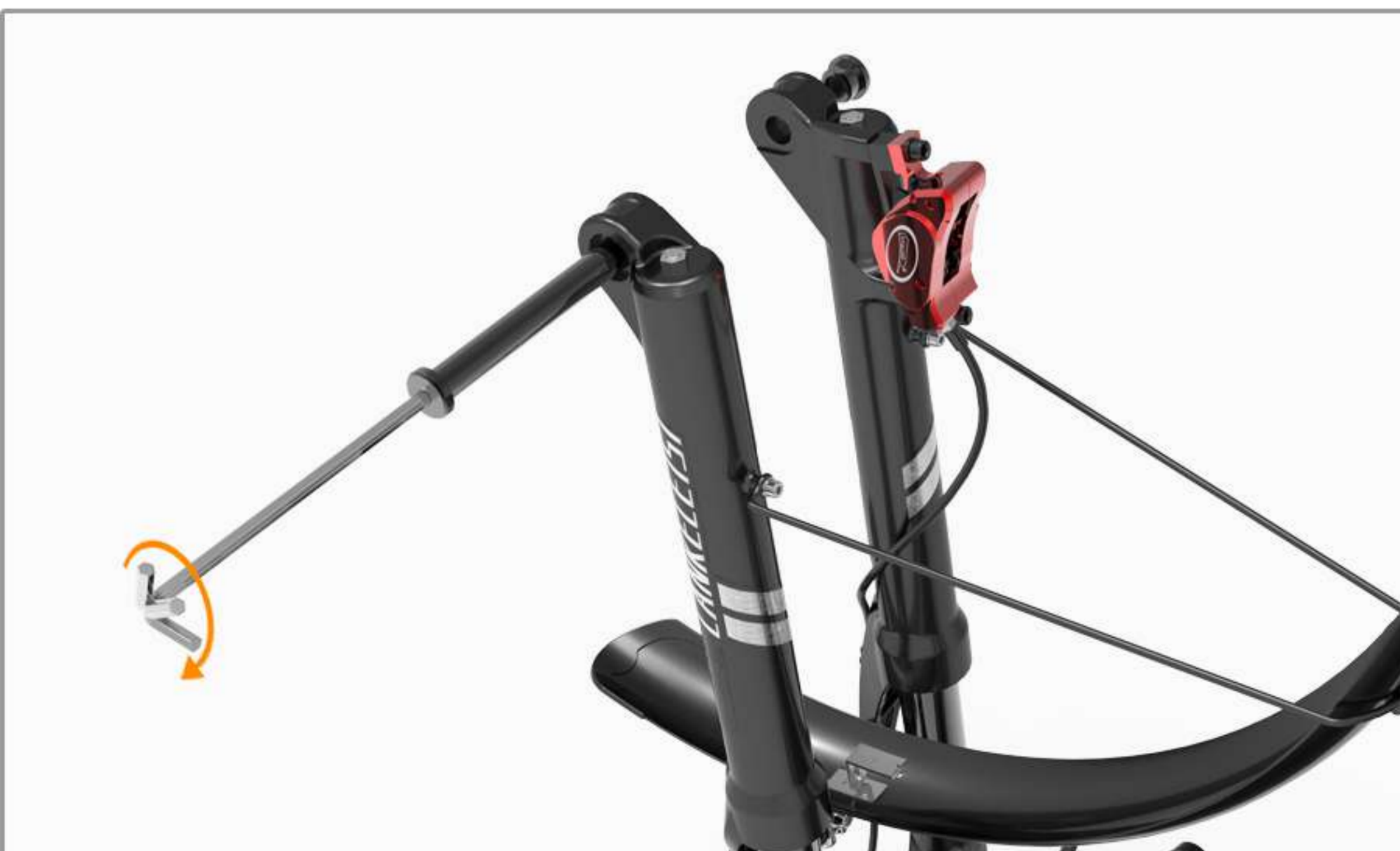
04 Remove front wheel mounting bearings
