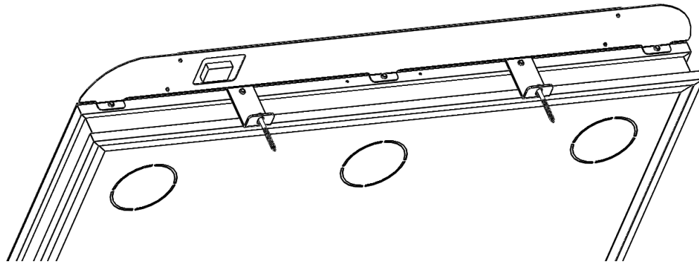
Figure 4: Long form solar panel bracket attached to the 1500 series heater walls.
