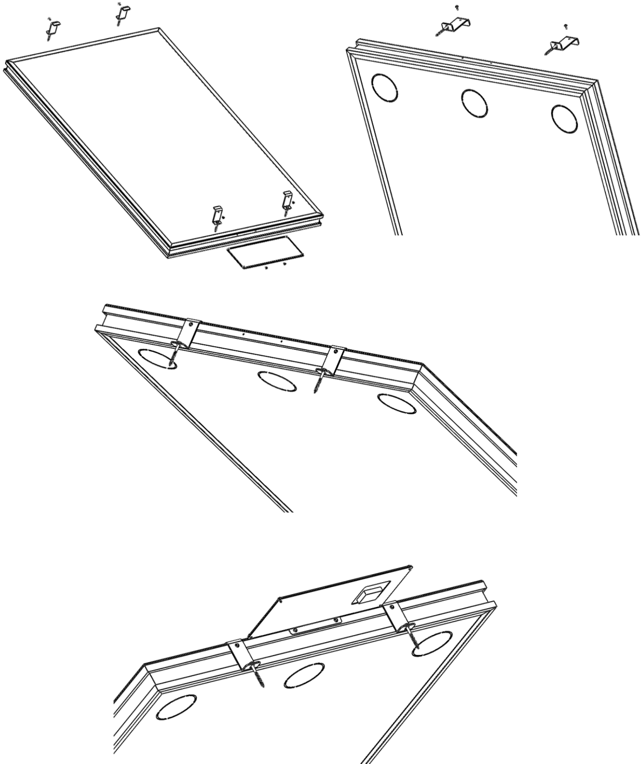
Figure 3: Exploded and collapsed views of the heater mounting brackets and standard solar panel bracket attached to the heater walls.
