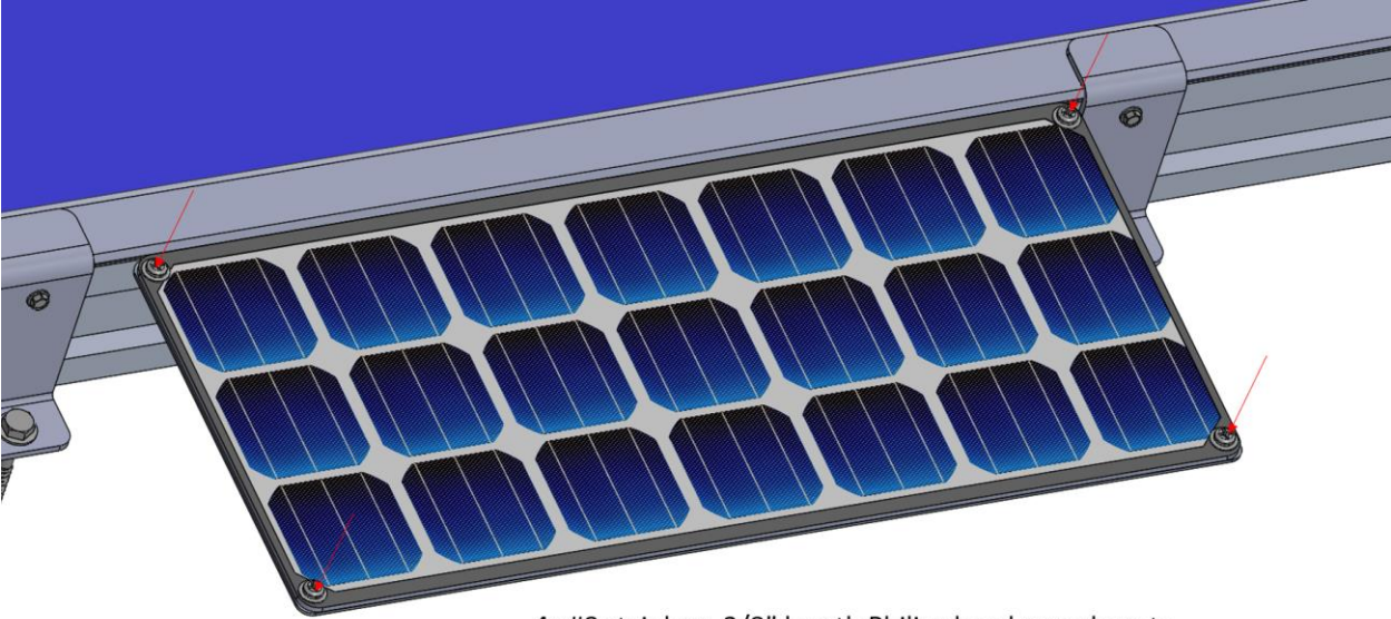
4x #8 stainless, 3/8" length Philips head + washers to connect solar panel to solar panel mounting bracket
