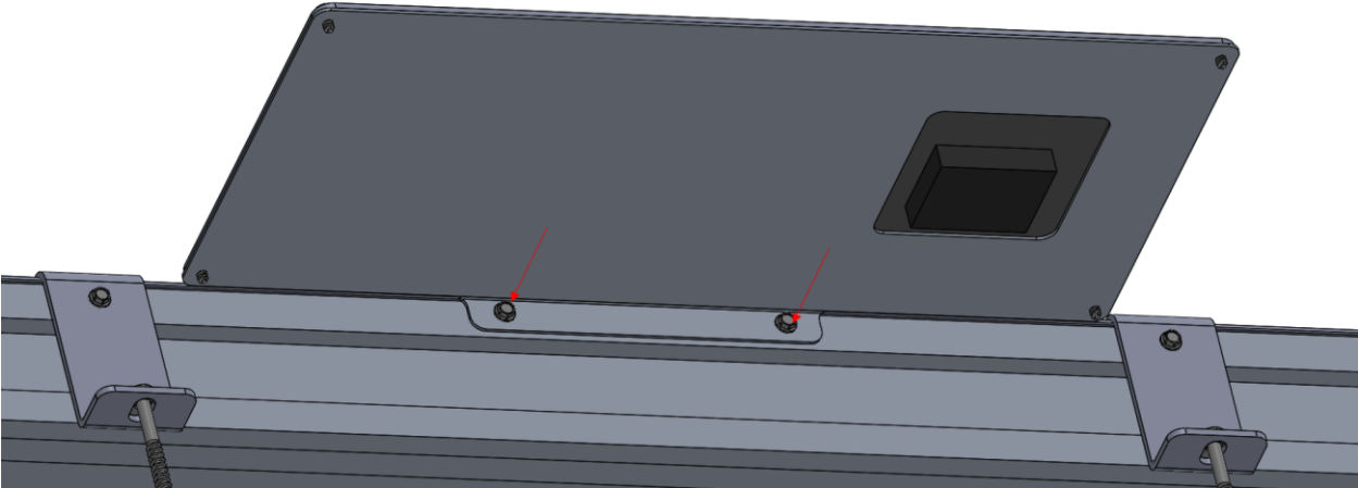
2x #8 stainless, 3/8" length hex head bolts to connect solar panel mounting bracket to top of heater bottom side rail
