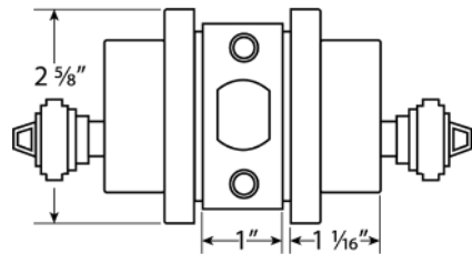
SQ-330 DOUBLE CYLINDER
