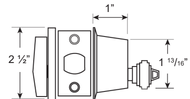
CB160 SINGLE CYLINDER
