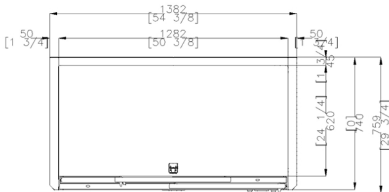
C-49RS TOP VIEW
