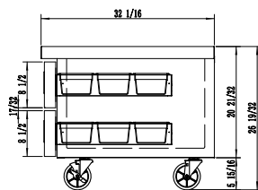
SIDE VIEW (1,2,3 DOORS)
