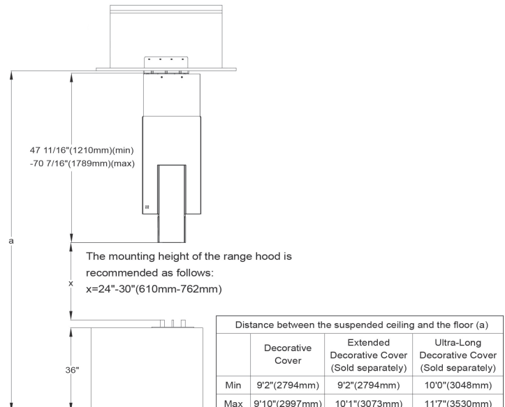
▼ Installation Dimensions
