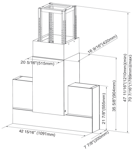
▼ Product Dimensions
