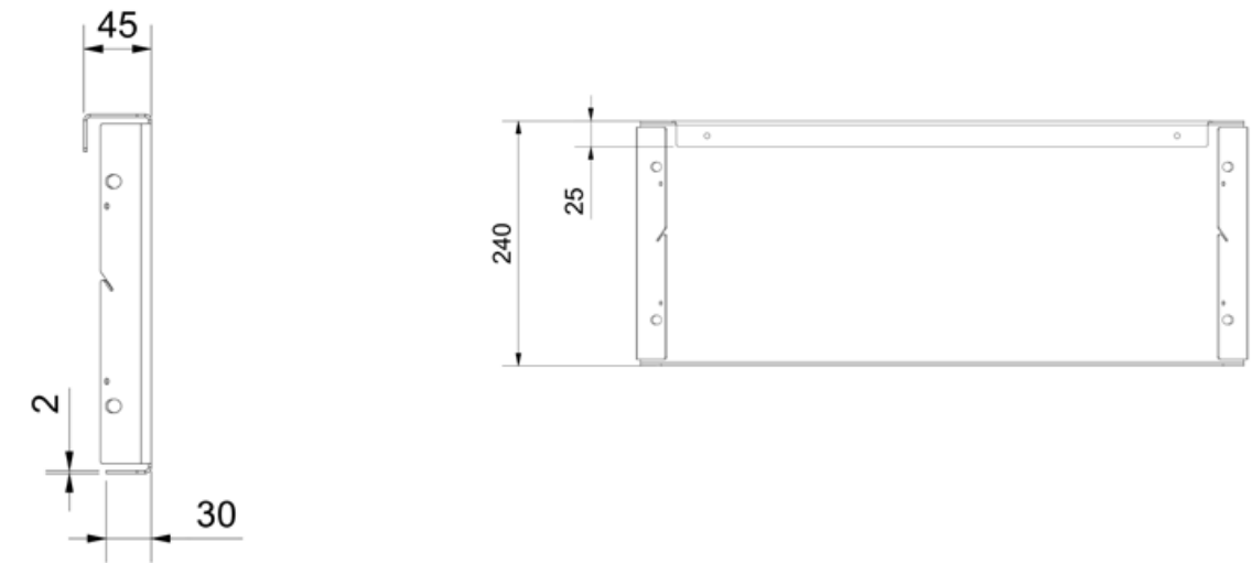
PANEL END/JOIN FLANGE
