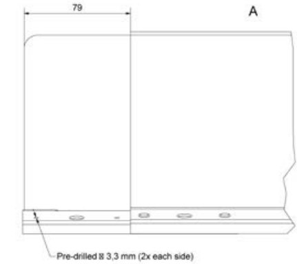
CONNECTOR PLATE
