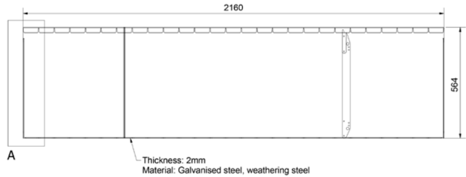
STRAIGHTCURVE® FLEX RAISED GARDEN BED PANEL - 560MM
