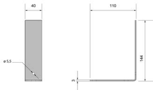
HARD SURFACE FIXING BRACKET
