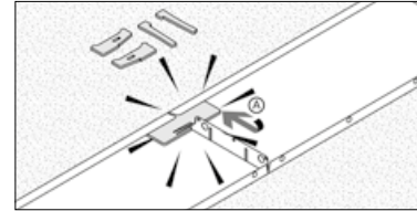
STEP 3 - Join using the joining set, break the pieces apart first by hand and insert join bracket ( A ) securely under the top lip (centered). Press it against back of panels (use a metal hammer to firmly lock in)
