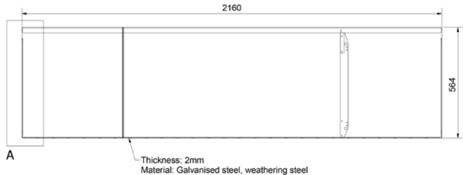
STRAIGHTCURVE® RIGID RAISED GARDEN BED PANEL - 560mm
