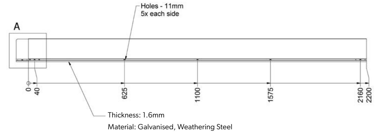
STRAIGHTCURVE® ZERO-FLEX GARDEN EDGING - 150MM
