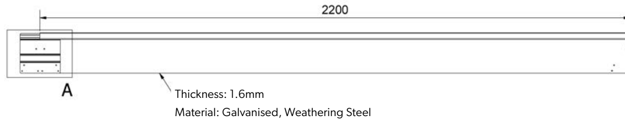
STRAIGHTCURVE® RIGID GARDEN EDGING - 150MM
