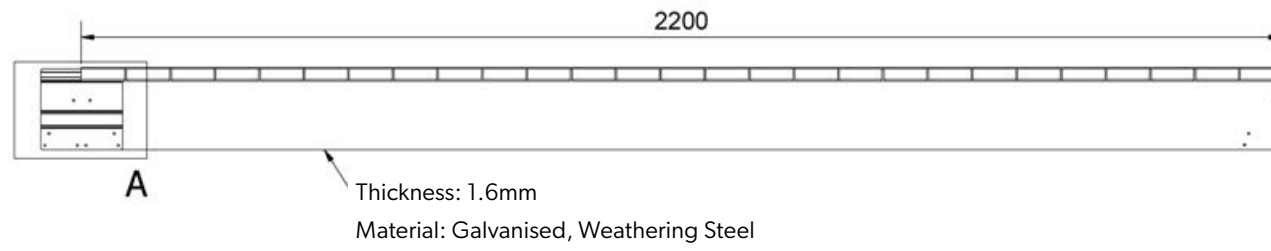
STRAIGHTCURVE® FLEX GARDEN EDGING - 150MM
