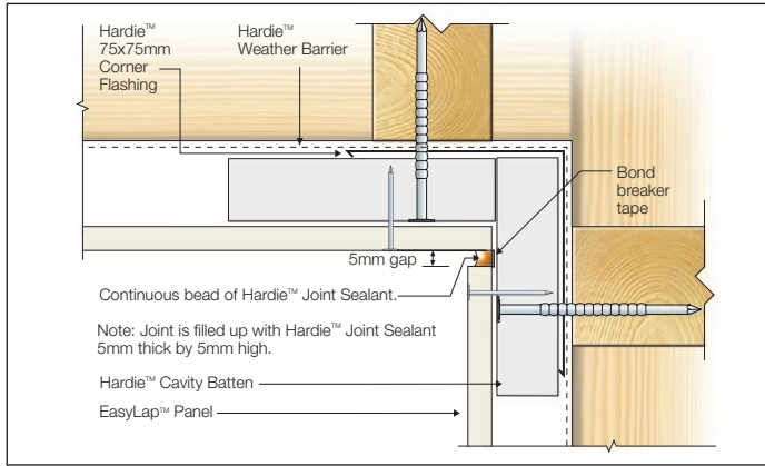
FIGURE 23 SEALANT FILL OPTION - CAVITY BATTEN
