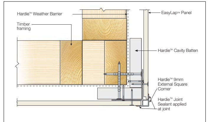
FIGURE 20 ALUMINIUM BOX CORNER OPTION - CAVITY BATTEN
