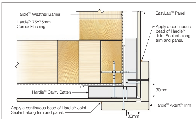
FIGURE 21 TRIM CORNER OPTION - CAVITY BATTEN
