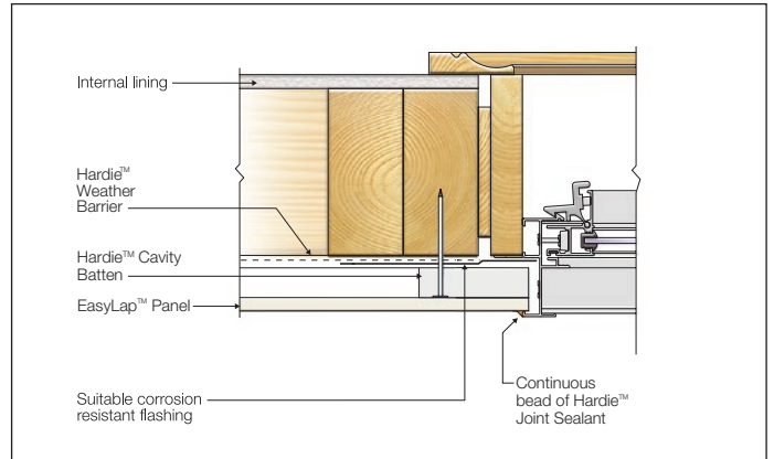
FIGURE 26 WINDOW JAMB - CAVITY BATTEN
