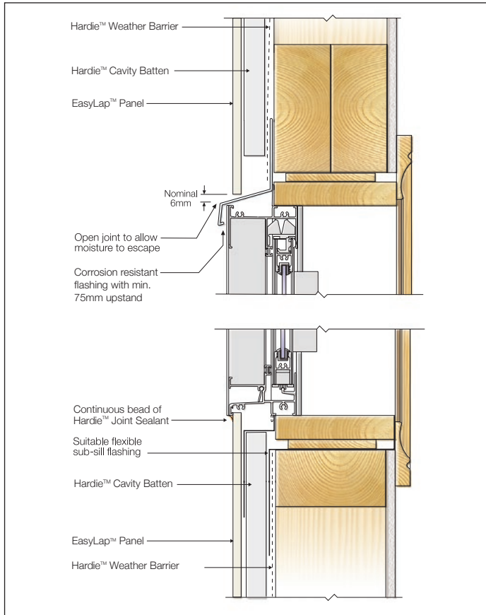
FIGURE 25 WINDOW HEAD AND SILL - CAVITY BATTEN
