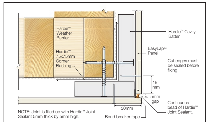
FIGURE 22 SEALANT FILL OPTION - CAVITY BATTEN
