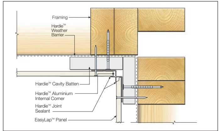
FIGURE 24 ALUMINIUM CORNER DETAIL - CAVITY BATTEN
