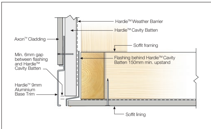
FIGURE 21 FAÇADE/SOFFIT JUNCTION
