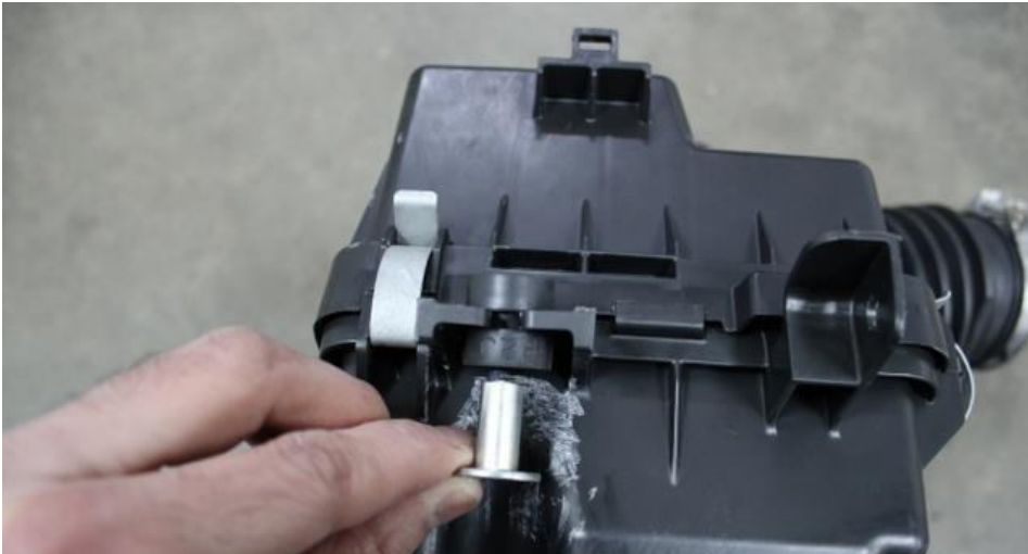
17. Rubber mounts can be removed by sliding out the metal bush and then squeezing out the rubber.
