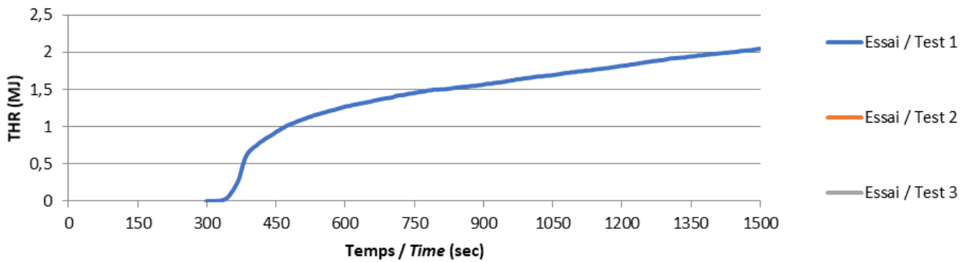
THR (t)
