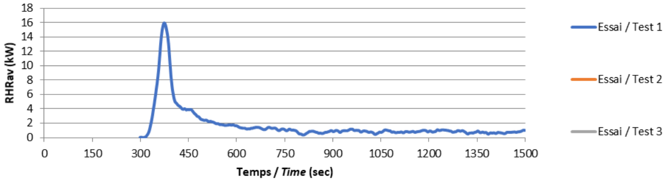
RHRav (t)
