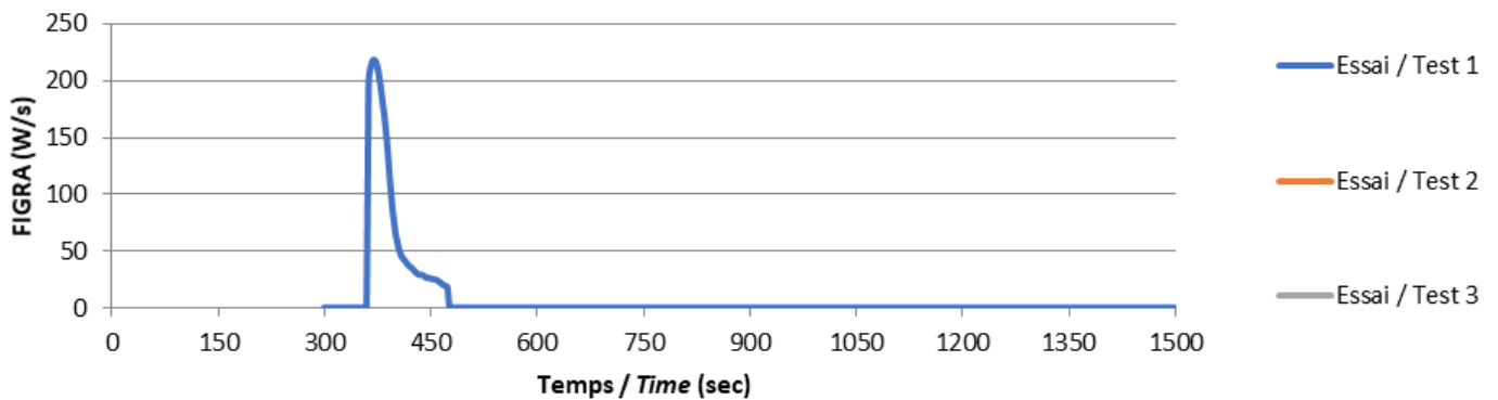
FIGRA (t)
