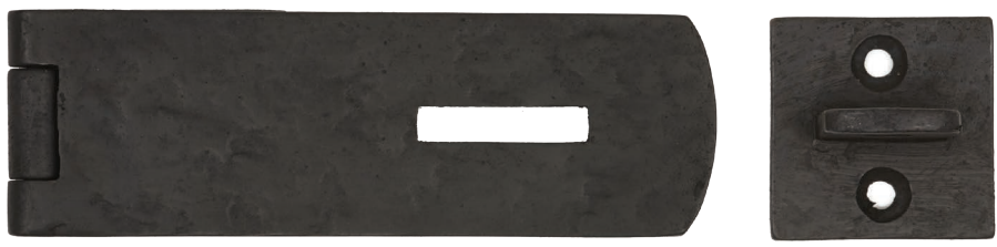
6" Lockable Hasp 50-450 Thickness: .20" / 5mm Screw: 1" Flat | #10 Stainless Dimensions: 6" L x 1-1/2" W Padlock Hole Diameter: 3/8"
