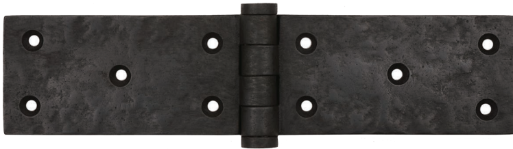
8-5/8" x 2" Bi-fold Hinge 30-435 Thickness: .275" / 6mm Screw: 1-1/4" Flat | #10 Stainless Weight Load (Pair): 75 Lbs
