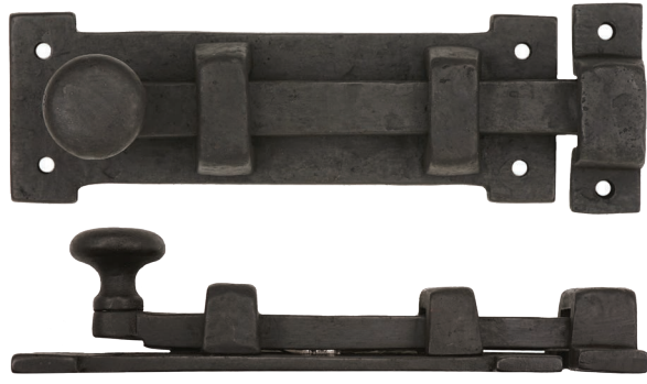
5" Surface Slide Bolt 90-105 Dimensions: 5" L x 3/4" W Screw: 1" Round | #10 Stainless Throw: 1" Total Included: (1) Slide Bolt, Catch (Shown)
