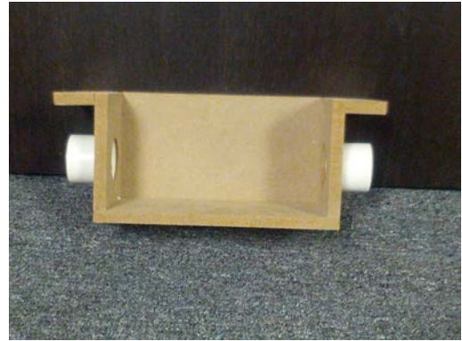
6c – Install collars into ball catch
