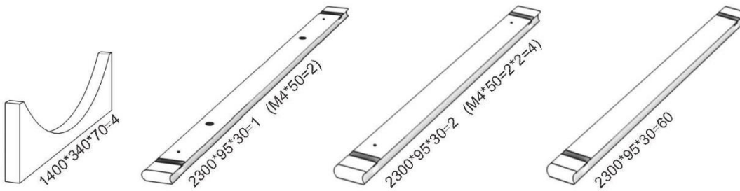
1 Cradles 2 The First bottom Stave (with two drain holes and 2 pre-drilled holes) 3 The 7th bottom staves (with 2 pre-drilled holes) 4 Standard staves
