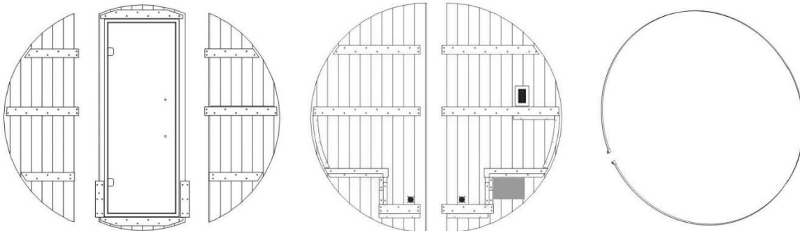
11 1794*791*30+20+19=1 1633*513.6+30*20=2(M4*40=12) Front wall panel 12 1794*905*30+20+20=2 (M4*40=6) Rear wall panel 13 5672*24*0.5=3 Stainless steel band
