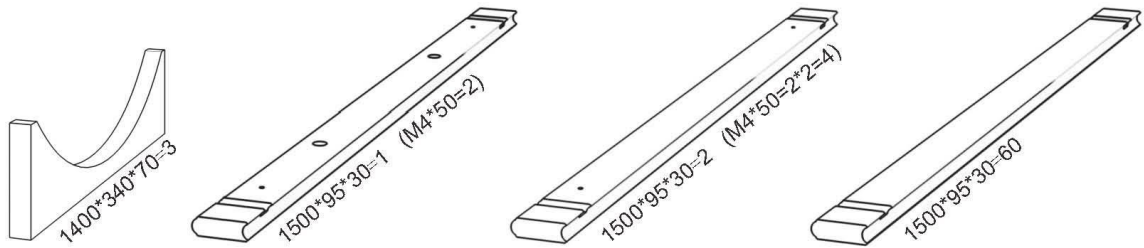
1 Cradles 2 The First bottom Stave (with two drain holes and 2 pre-drilled holes) 3 The 7th bottom staves (with 2 pre-drilled holes) 4 Standard staves
