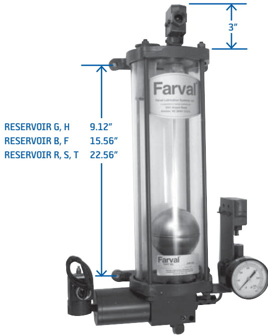
TS30-TKEXA Station with Pump, Reservoir and Accessories
