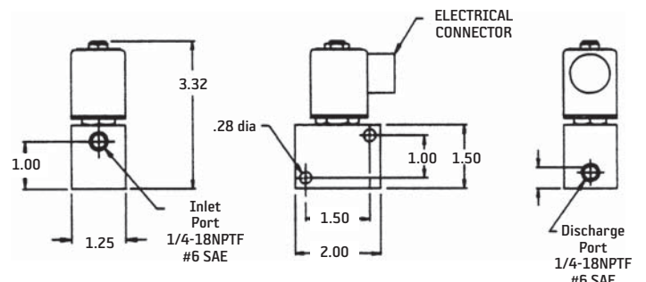
Oil Service (MCZ2501 Series)
