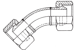
Female (CS) 45° Swept Elbow
