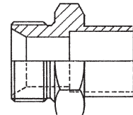
Hex Male for Socket Weld Tube 'CS'
