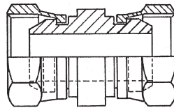
Female/Female (CS) Adaptor
