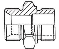
Male (CS) x Male (OR) Adaptor SAE
