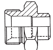
Hex Male for Butt Weld Tube 'CS'
