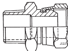
Swivel Female x Taper Male Adaptor BSP'T'
