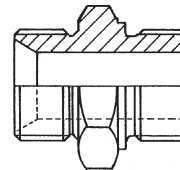
Male (CS) x Male (OR) Adaptor BSP'P'
