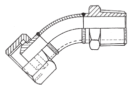
Male Taper 45° Swept Elbow BSP'T'
