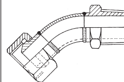
Male Taper 45° Swept Elbow NPT
