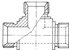
Male (CS) Tee
