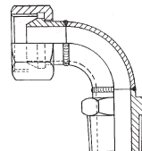
Male Taper 90° Swept Elbow BSP'T'
