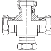
Female (CS) Cross
