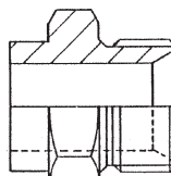
Fixed Male 'CS'
