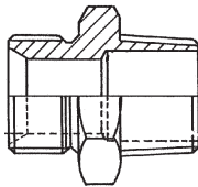
Male (CS) x Taper Adaptor NPT
