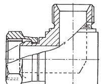
90° Swivel Nut Elbow
