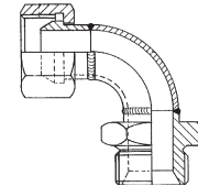
90° Swivel Nut Swept Elbow
