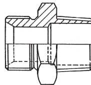
Male (CS) x Taper Adaptor BSP'T'
