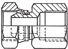
Swivel Female x Fixed Female SAE
