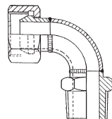
Male Taper 90° Swept Elbow NPT
