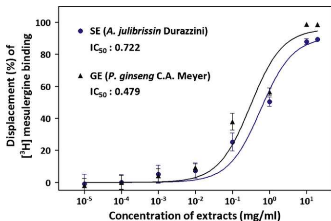
Fig. 2. Dose–response curves and IC 50 values of SE (silk tree, Albizzia julibrissin Durazzini) and GE (ginseng, Panax ginseng C.A. Meyer) in the 5-HT 2C receptor binding assay. Each data point is expressed as mean ± SD (n = 3).
