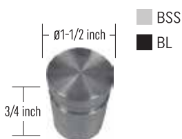
⇒ ISO11234C SS 316 Standoff Base With Cap 1-1/2" Dia x 3/4"
