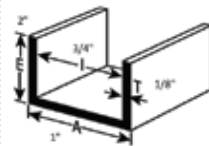
ICUCH21 2" Deep U-Channel 144" Length
