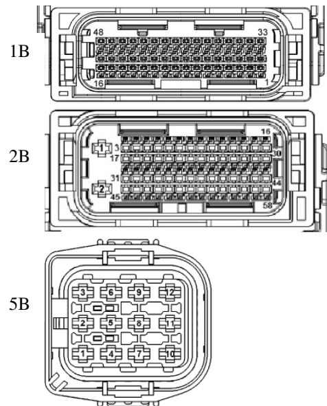
Terminal Side View of Connectors
