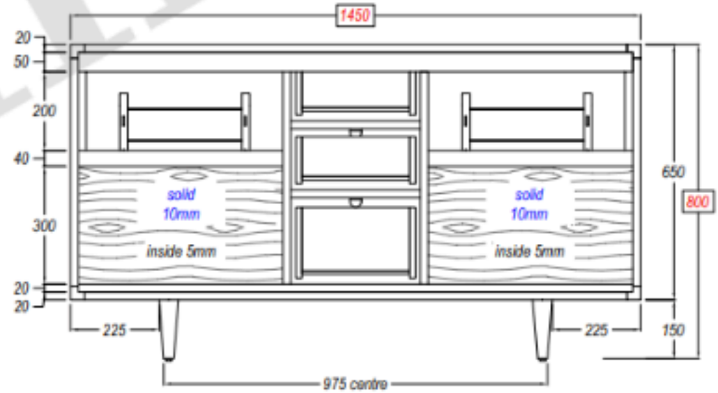
REAR VIEW Tampak Belakang
