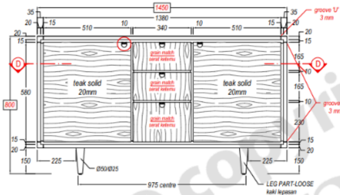
FRONT VIEW Tampak Muka
