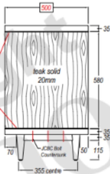
SIDE VIEW Tampak Samping
