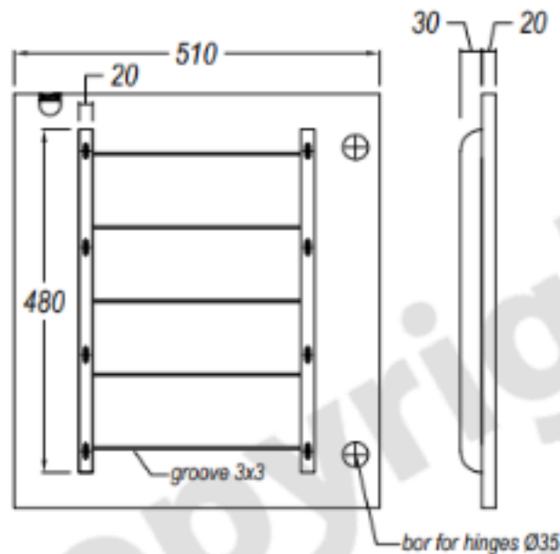
REAR VIEW-DOOR
