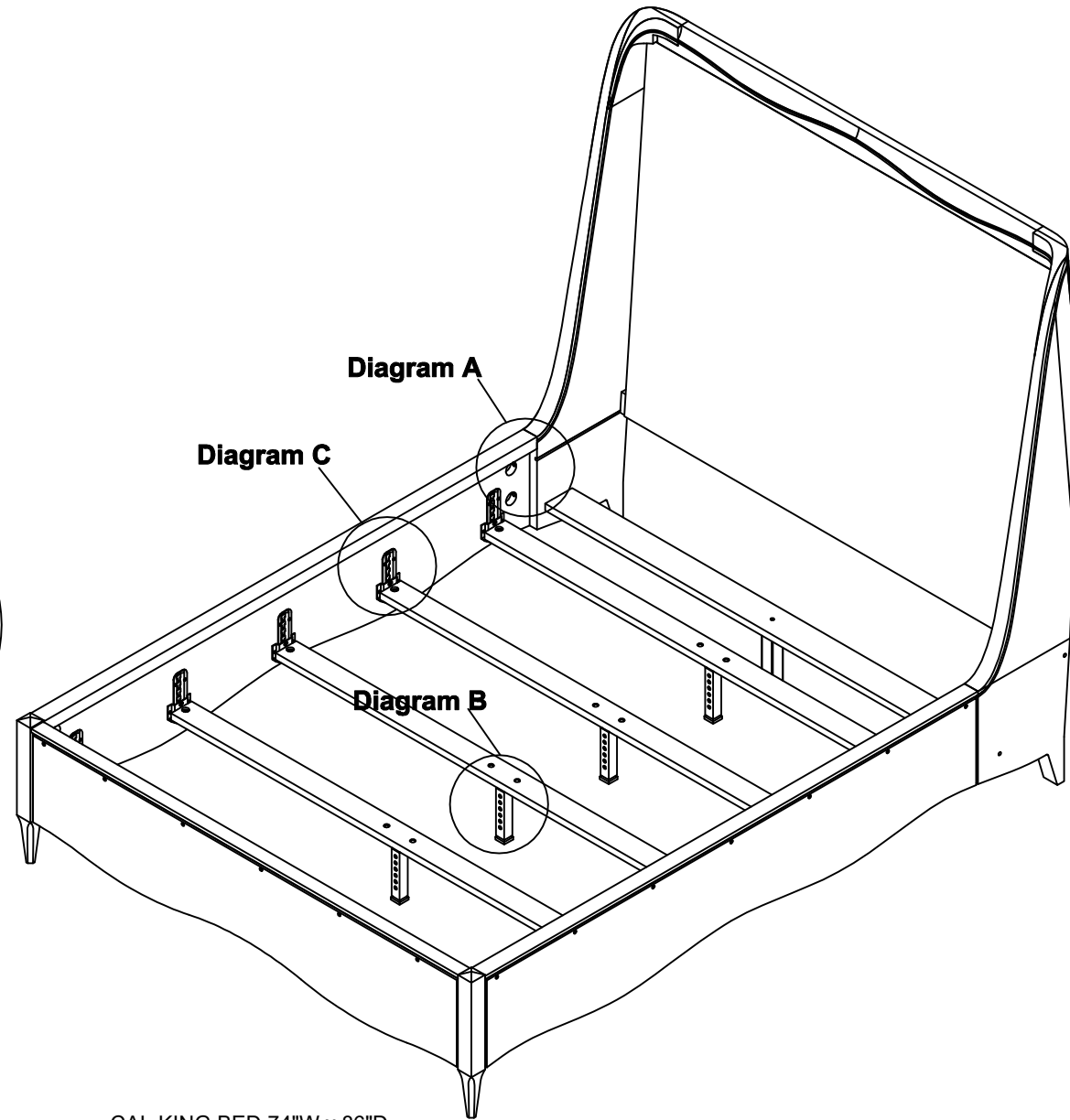
Adjustable Support Legs
