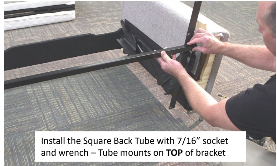
Install 4 bolts on each side. Back Support Tube is attached using the 2 nd hole from the bottom
