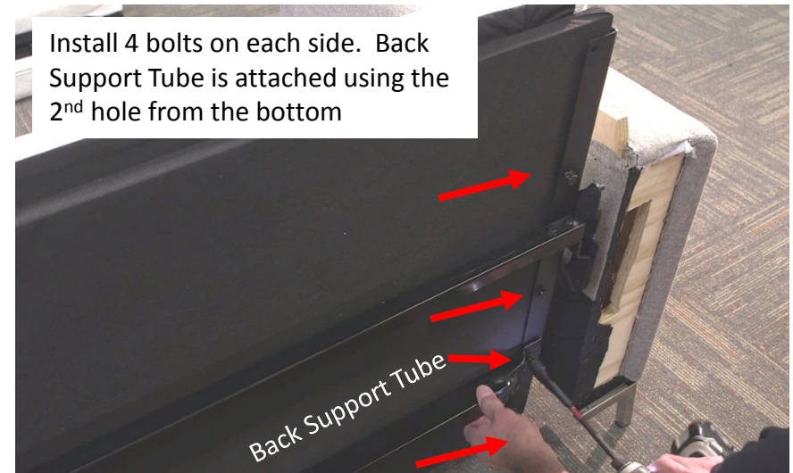
Install the Square Back Tube with 7/16" socket and wrench – Tube mounts on TOP of bracket
