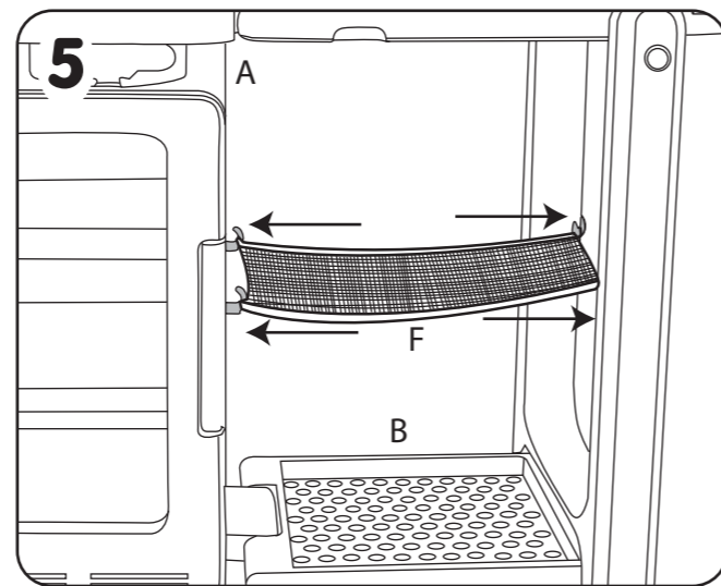
Hang the net (F) on the hooks above the tray (B).
