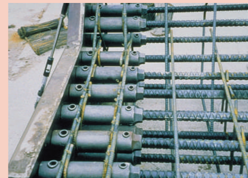
The taper threaded sleeve keeps the bar in axial alignment to increase field tolerance of the rebar dowels.
