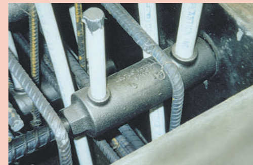
Standard 1/2" (13 mm) and 3/4" (19 mm) PVC or flexible tubing is used for the inlet and outlet ports.
