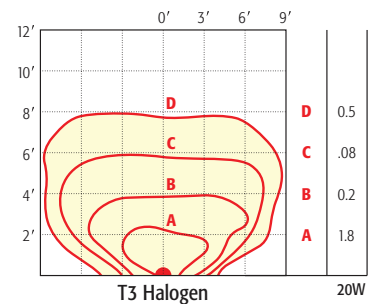
Horizontal Foot Candle Full Spread
