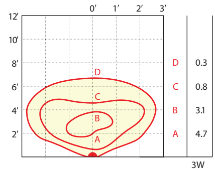
Horizontal Foot Candle Full Spread
