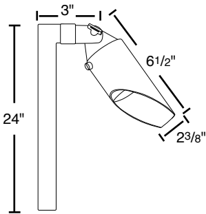
1/2" npt Dimensions (inch)
