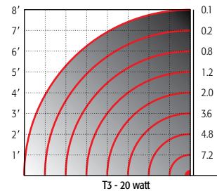
Horizontal Foot Candle Quarter Beam Spread
